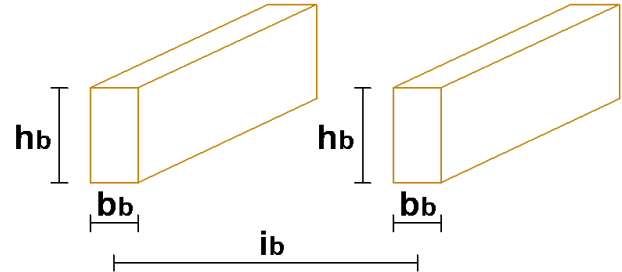
Figure: geometric characteristics of the floor
