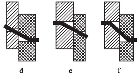
Figure: Failure modes for timber and panel connections.
