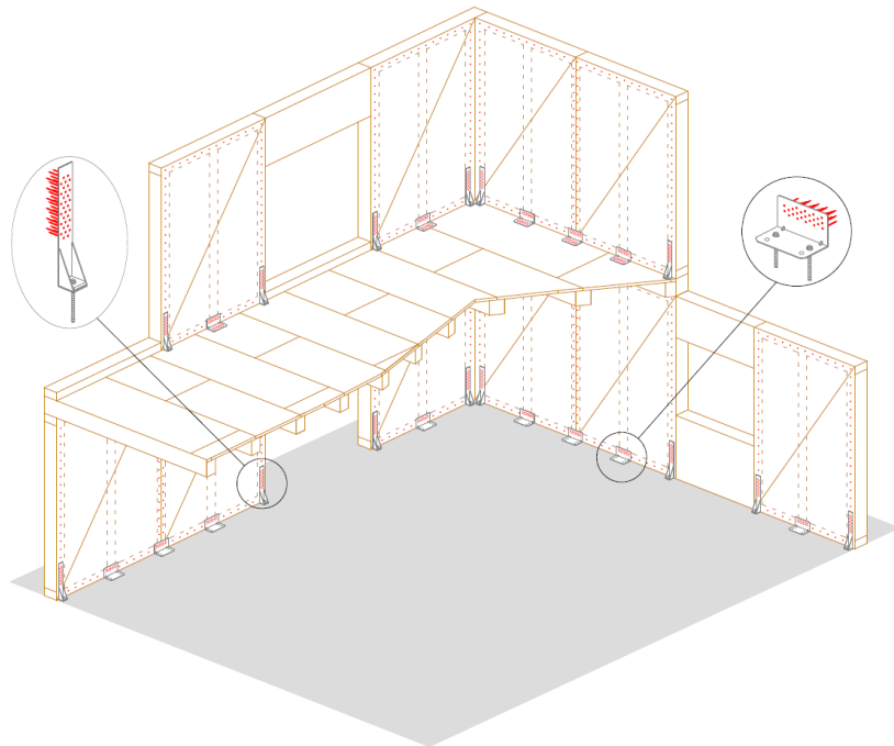
Figure 1 - Light timber frame building in ductility class DCM: dissipative zones
