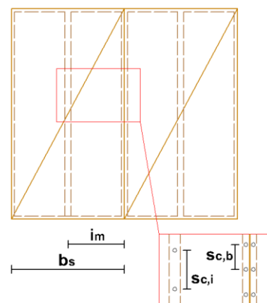
Figure: dimensions of the sheeting boards and fasteners spacing
